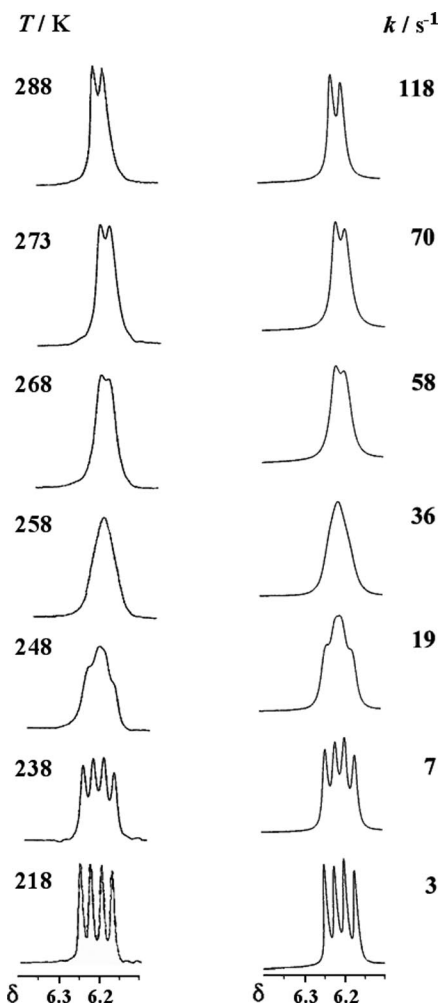
Figure 1. Variable-temperature spectra of an equimolar mixture of [\text{Rh}(\text{phpy})_2\{\text{H}_2(\text{isopropyl})_2\text{C}_2\text{N}_2\text{S}_2 \kappa\text{-S,S-Rh}\}]^+\text{Cl}^- ( 2 ) and [\text{Rh}(\text{phpy})_2\{\text{H}(\text{isopropyl})_2\text{C}_2\text{N}_2\text{S}_2 \kappa\text{-S,S-Rh}\}] ( 6 ) in the 6.1–6.4 ppm region. Computer-synthesized spectra are shown on the right.
