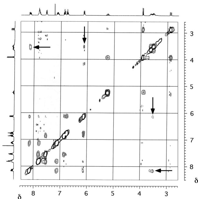
Figure 3. NOESY spectrum of [\text{Rh}(\text{phpy})_2\{\mu\text{-(isoamyl)}_2\text{-C}_2\text{N}_2\text{S}_2\}\text{Pd}(\eta^3\text{-allyl})\kappa\text{-N,N-Rh}\kappa\text{-S,S-Pd}]\text{ (14)} . Cross peaks marked with horizontal arrows indicate the proximity of the \text{N-CH}_2 protons to \text{H}^6 of 2-phenylpyridine; the peaks indicated by vertical arrows refer to the polar interaction between \text{N-CH}_2 and \text{H}^{6'} of 2-phenylpyridine.
