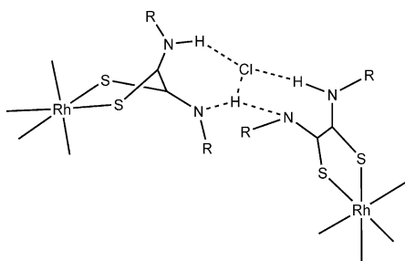
Figure 2. Proposed transition state for the HCl exchange process between the ion pair [\text{Rh}(\text{phpy})_2(\text{H}_2\text{R}_2\text{C}_2\text{N}_2\text{S}_2 \kappa\text{-S,S-Rh})]^+\text{Cl}^- ( \text{H}_2\text{R}_2\text{C}_2\text{N}_2\text{S}_2 = dialkyldithiooxamide) and [\text{Rh}(\text{phpy})_2(\text{HR}_2\text{C}_2\text{N}_2\text{S}_2 \kappa\text{-S,S-Rh})] .
