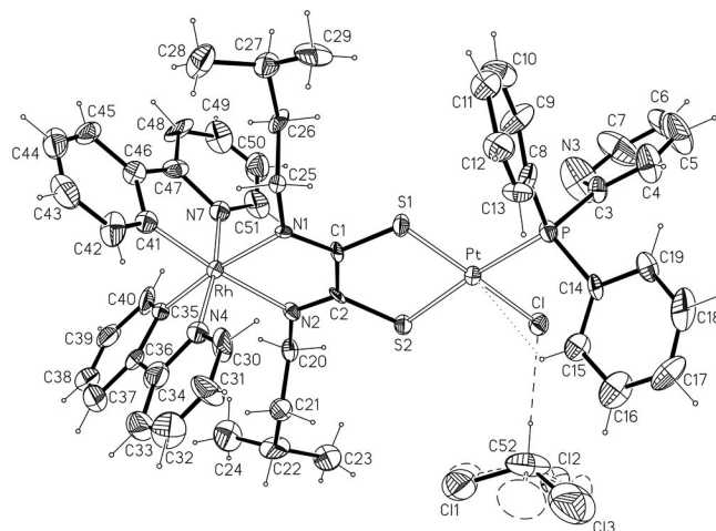
Figure 5. Asymmetric unit of the crystal model of 16 obtained by single-crystal X-ray diffraction, showing the molecular geometry and co-crystallized chloroform in a ratio of 1:1. Thermal ellipsoids are at the 25% probability level, while the H size is arbitrary. Selected bond lengths [Å] and angles [°]: \text{Pt-P} = 2.258(6) , \text{Pt-S1} = 2.271(5) , \text{Pt-S2} = 2.315(5) , \text{Pt-Cl} = 2.336(5) , \text{Rh-C35} = 1.97(2) , \text{Rh-N4} = 2.00(2) , \text{Rh-N7} = 2.01(2) , \text{Rh-C41} = 2.01(2) , \text{Rh-N1} = 2.15(2) , \text{Rh-N2} = 2.17(1) , \text{S1-Pt-S2} = 89.6(2) , \text{N1-Rh-N2} = 75.9(6) , \text{N7-Rh-C41} = 84.3(8) , \text{C35-Rh-N4} = 84.2(8) , \text{S1-Cl} = 1.74(2) , \text{S2-C2} = 1.77(2) , \text{C1-N1} = 1.33(2) , \text{C1-C2} = 1.44(2) , \text{S1-C1-C2-S2} = 2(2) .
