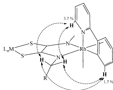
Figure 4. Schematic view of the polar interactions between the \alpha hydrogen atoms of the alkyl substituents of the dithiooxamide ligand and the \text{H}^6 and \text{H}^{6'} protons of the \text{N,C} -coordinated 2-phenylpyridine. Each \text{N-CH}_2 group is equidistant from the \text{H}^6 and \text{H}^{6'} protons of both 2-phenylpyridine moieties. Irradiation of the \text{N-CH}_2 protons enhances the signal for \text{H}^6 (ca. 3.7%) and that for \text{H}^{6'} (ca. 1.7%) in all the bimetallic complexes 13–16 .
